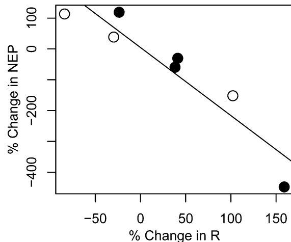
Figure 6. Relationship between storm responses of respiration and net ecosystem production. The relationship between changes in respiration ( R ) and changes in net ecosystem production (NEP) following Irene (% change in NEP = -2.2 \times % change in R + 4.6, p = 0.002 , r^2 = 0.87 ). Change in metabolism parameters are the percent difference between the 10 day mean after Irene and the 10 day mean before Irene. Each point represents one lake, where open circles denote lakes with high potential volume replacement and closed circles are those with low potential volume replacement (see Figure 3). Metabolism estimates are available for seven of the nine lakes.
